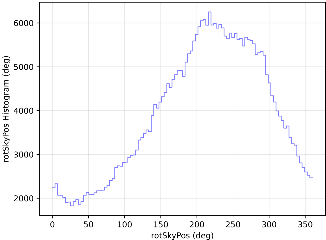
too_elab_r32_d3_gz_v3.4_10yrs All sky y band: rotSkyPos Histogram
