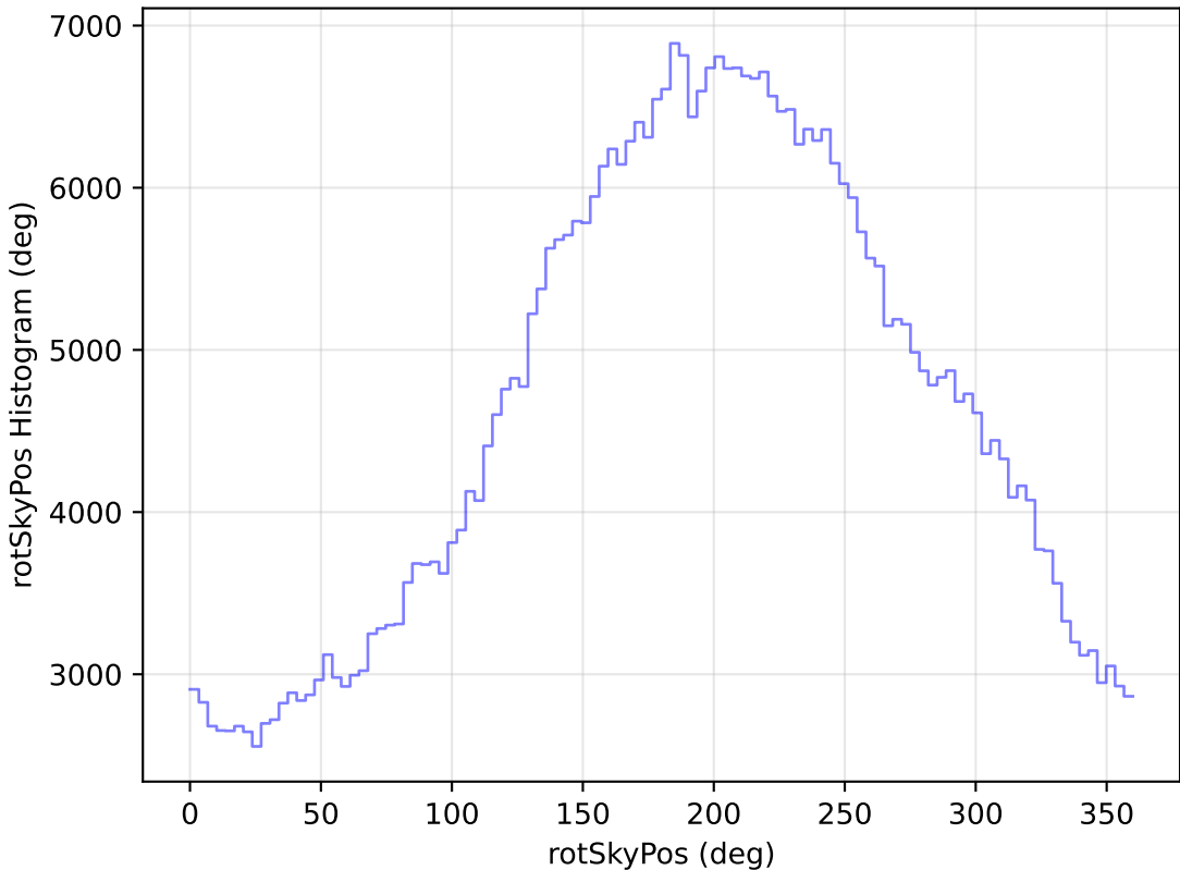
too_elab_r32_d3_gz_v3.4_10yrs All sky r band: rotSkyPos Histogram
