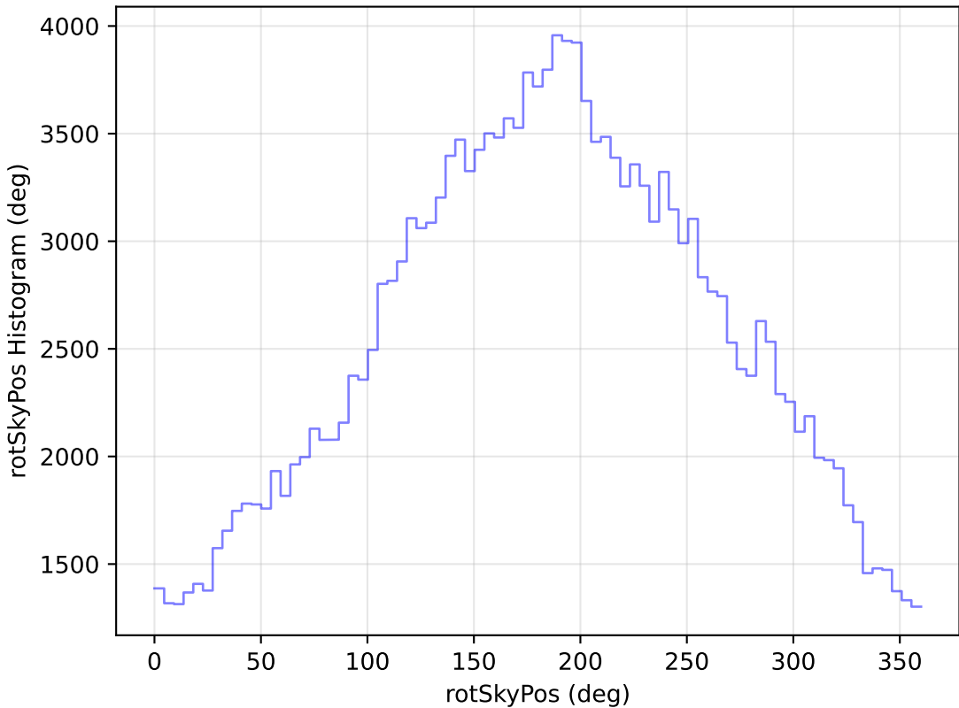
too_elab_r32_d3_gz_v3.4_10yrs All sky g band: rotSkyPos Histogram
