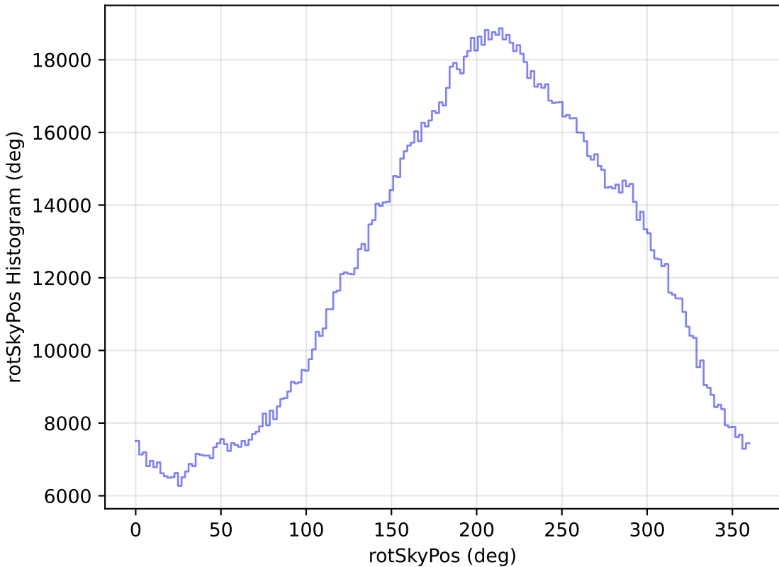
too_elab_r32_d3_gz_v3.4_10yrs All sky all bands: rotSkyPos Histogram
