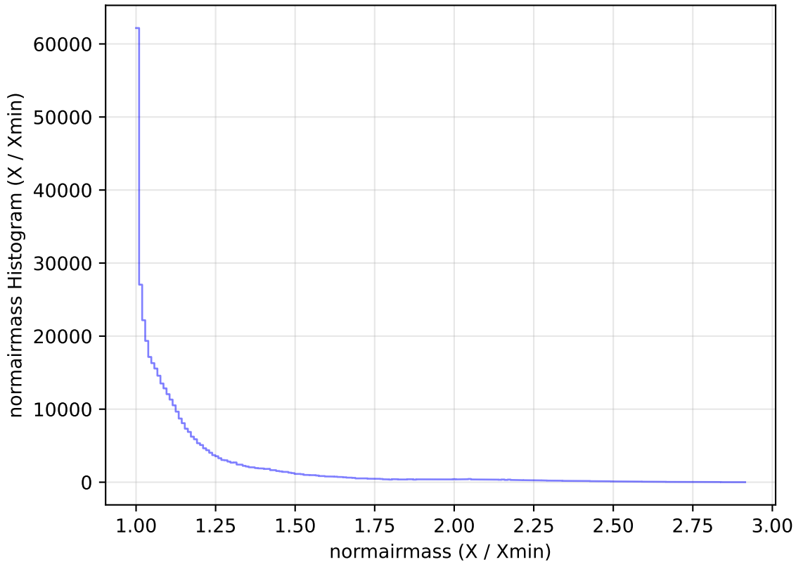
too_elab_r32_d3_gz_v3.4_10yrs WFD z band: normairmass Histogram
