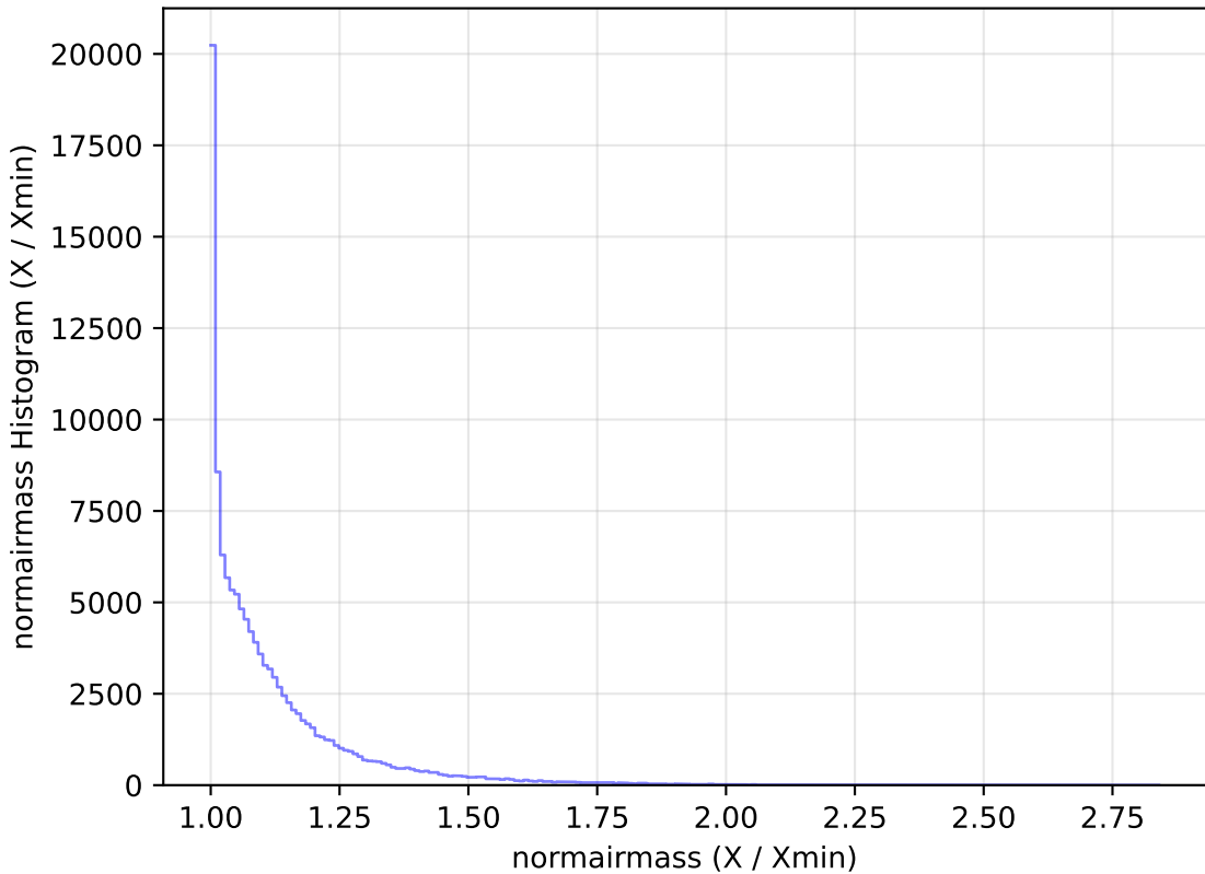
too_elab_r32_d3_gz_v3.4_10yrs WFD u band: normairmass Histogram
