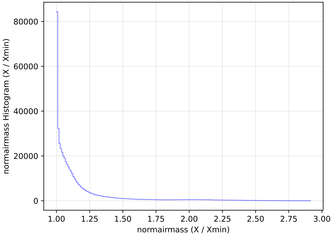
too_elab_r32_d3_gz_v3.4_10yrs WFD i band: normairmass Histogram
