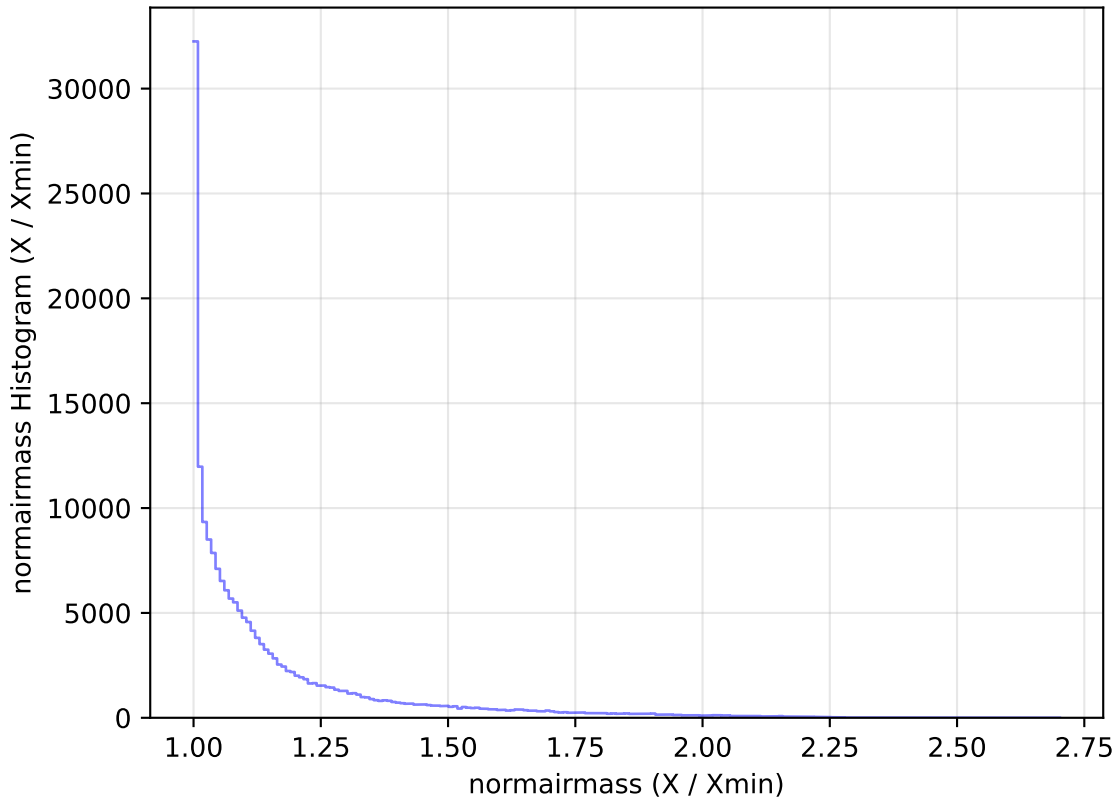
too_elab_r32_d3_gz_v3.4_10yrs WFD g band: normairmass Histogram
