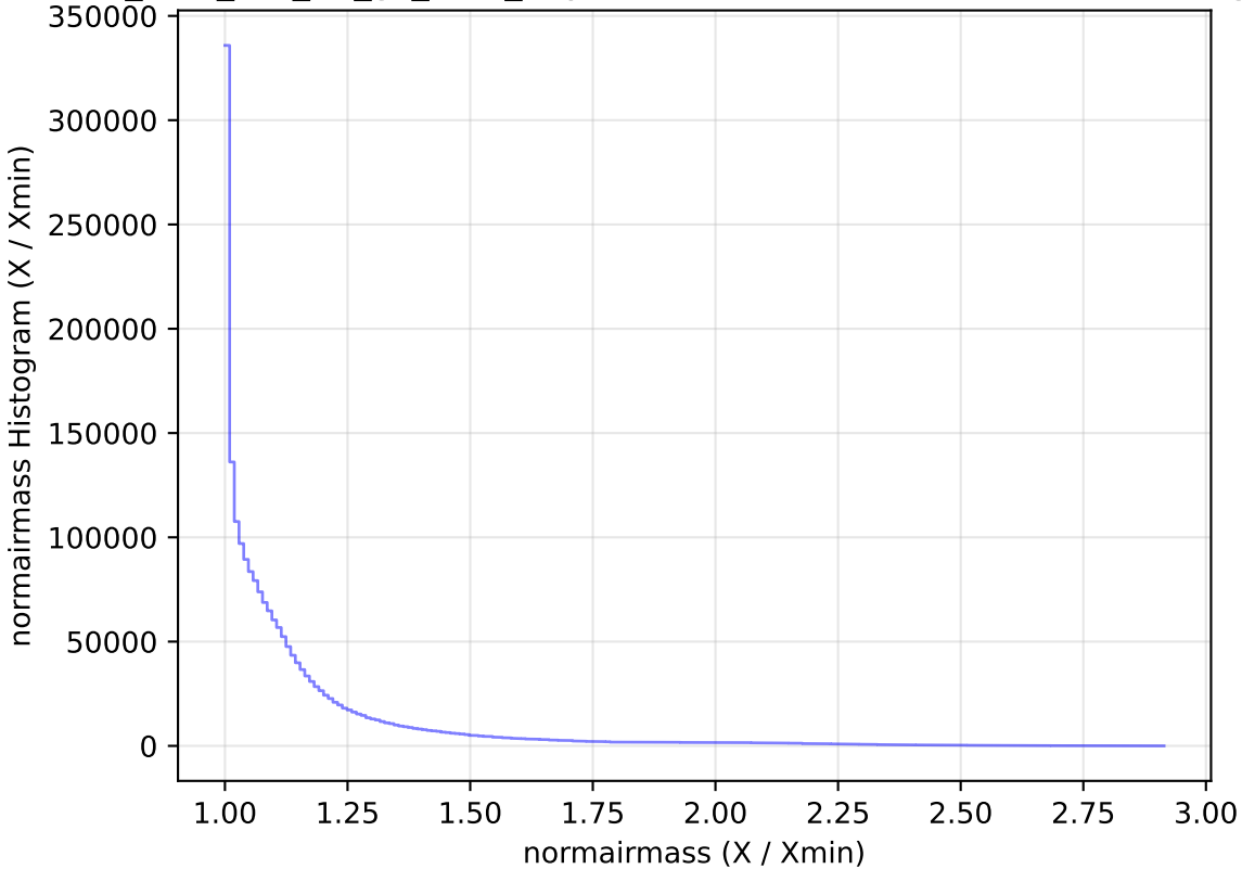
too_elab_r32_d3_gz_v3.4_10yrs WFD all bands: normairmass Histogram
