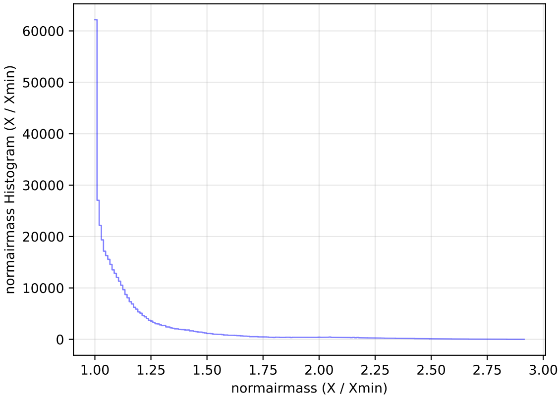
too_elab_r32_d3_gz_v3.4_10yrs All sky z band: normairmass Histogram
