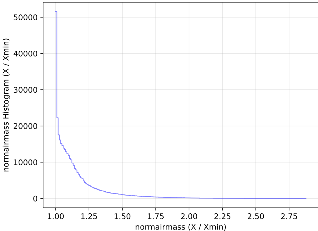
too_elab_r32_d3_gz_v3.4_10yrs All sky y band: normairmass Histogram
