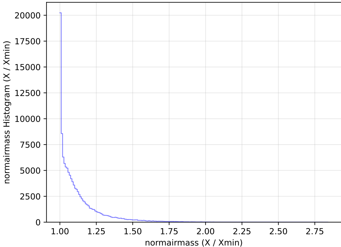
too_elab_r32_d3_gz_v3.4_10yrs All sky u band: normairmass Histogram
