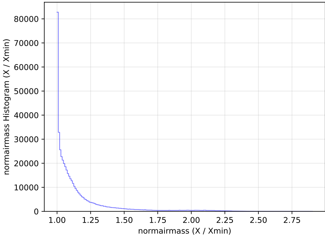
too_elab_r32_d3_gz_v3.4_10yrs All sky r band: normairmass Histogram
