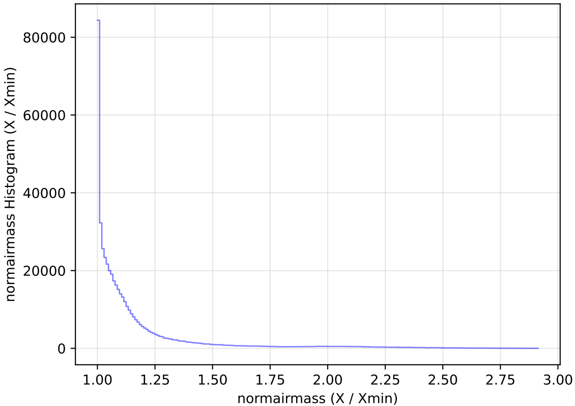
too_elab_r32_d3_gz_v3.4_10yrs All sky i band: normairmass Histogram
