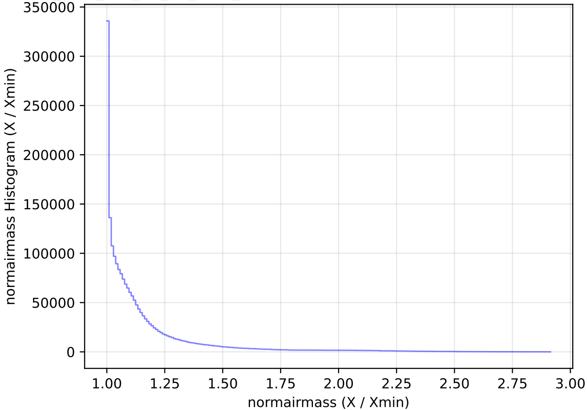
too_elab_r32_d3_gz_v3.4_10yrs All sky all bands: normairmass Histogram
