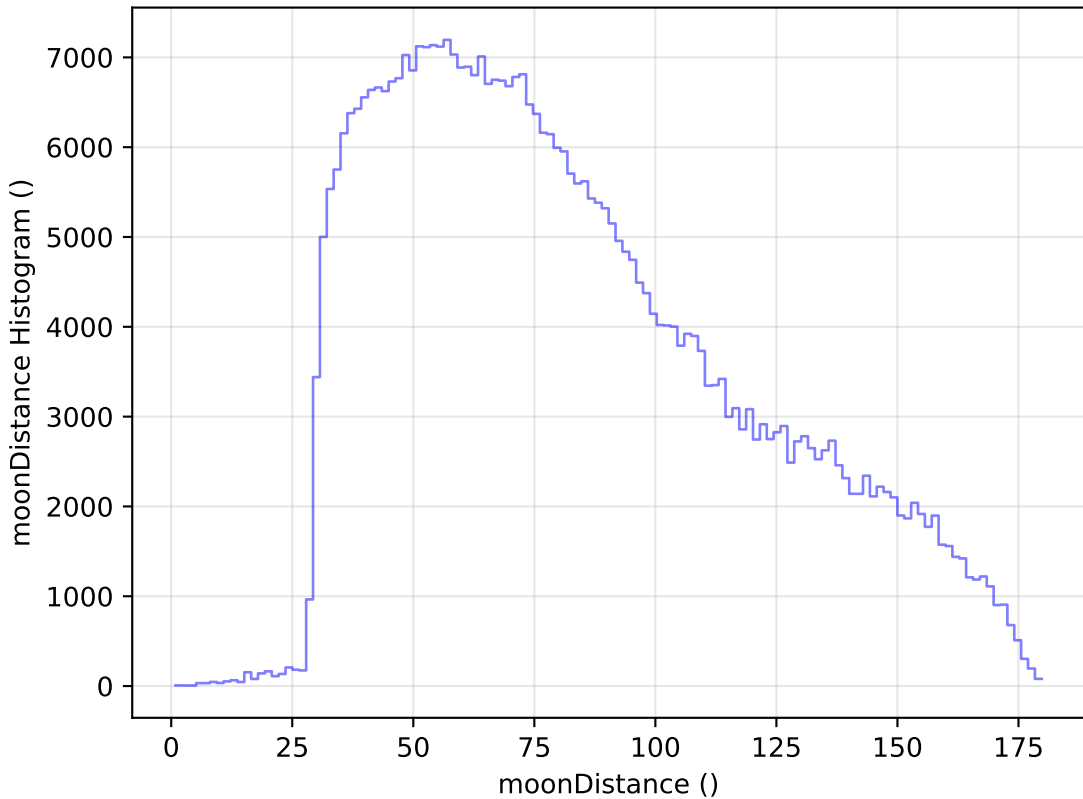
too_elab_r32_d3_gz_v3.4_10yrs WFD z band: moonDistance Histogram
