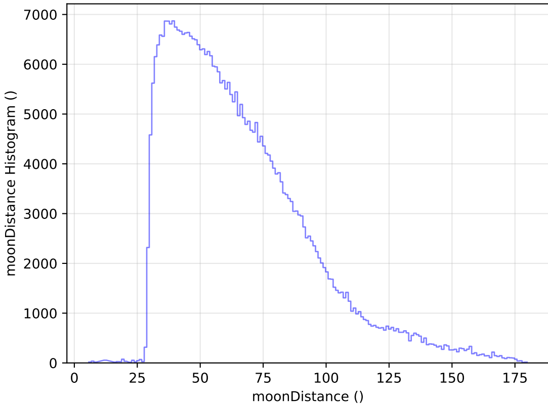
too_elab_r32_d3_gz_v3.4_10yrs WFD y band: moonDistance Histogram
