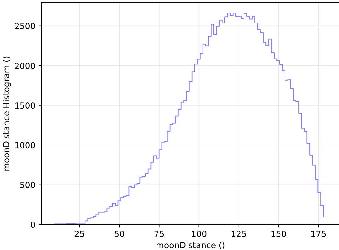
too_elab_r32_d3_gz_v3.4_10yrs WFD u band: moonDistance Histogram
