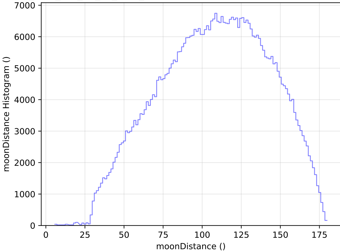
too_elab_r32_d3_gz_v3.4_10yrs WFD r band: moonDistance Histogram
