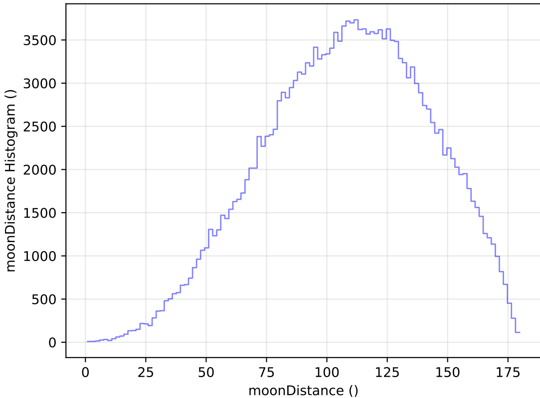
too_elab_r32_d3_gz_v3.4_10yrs WFD g band: moonDistance Histogram
