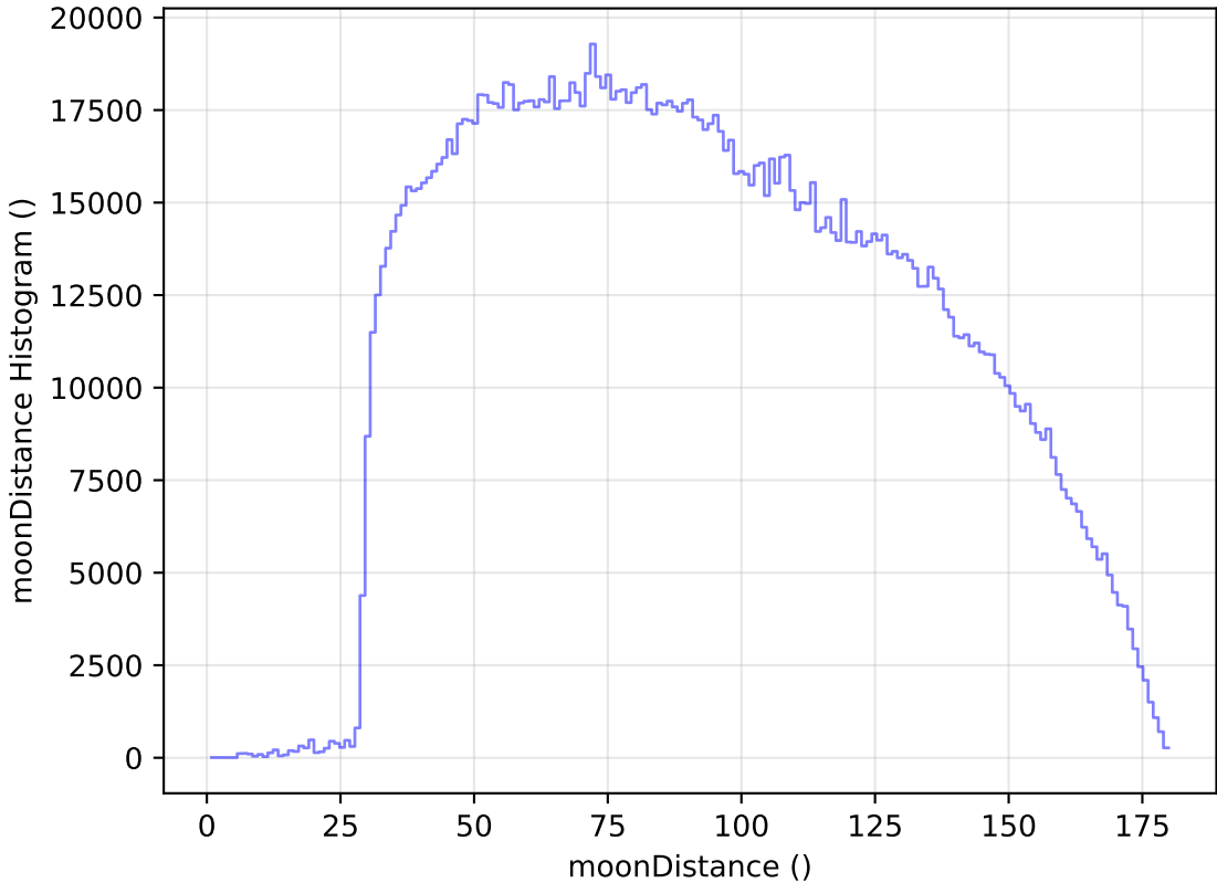
too_elab_r32_d3_gz_v3.4_10yrs WFD all bands: moonDistance Histogram
