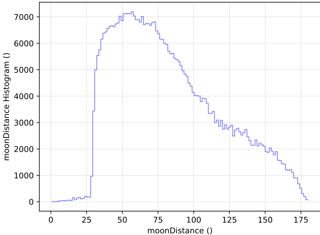
too_elab_r32_d3_gz_v3.4_10yrs All sky z band: moonDistance Histogram
