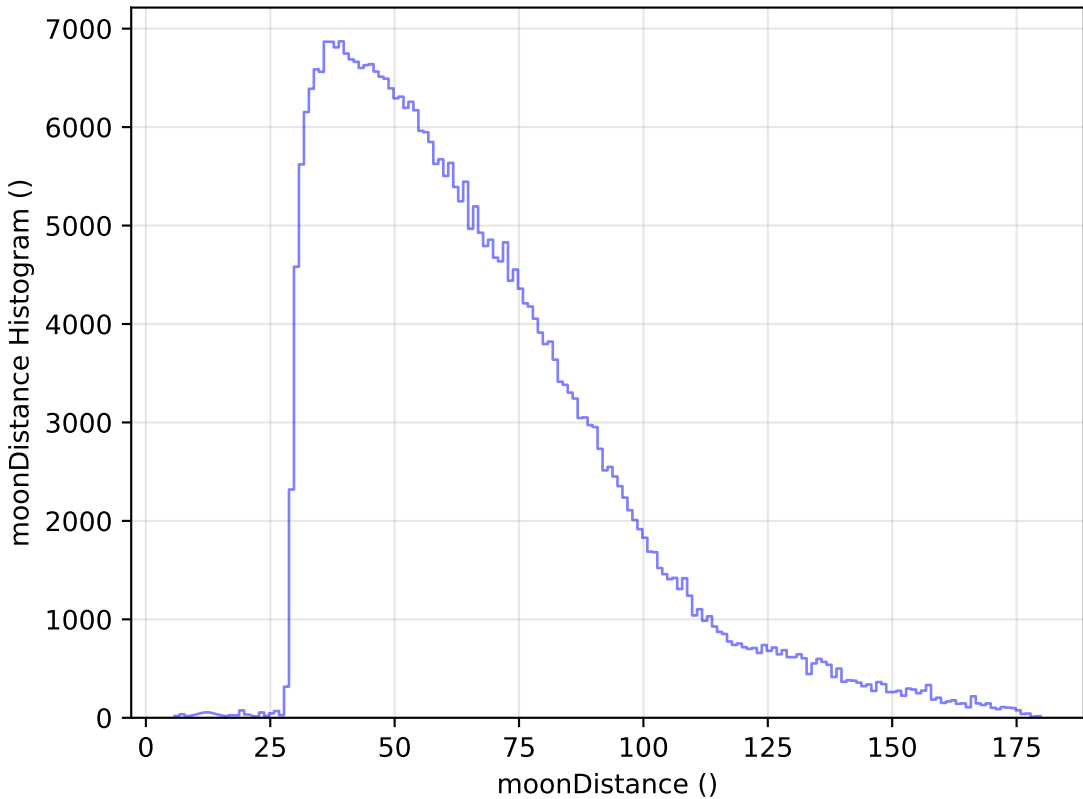
too_elab_r32_d3_gz_v3.4_10yrs All sky y band: moonDistance Histogram
