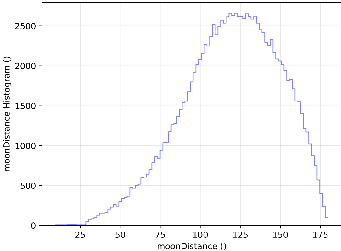
too_elab_r32_d3_gz_v3.4_10yrs All sky u band: moonDistance Histogram
