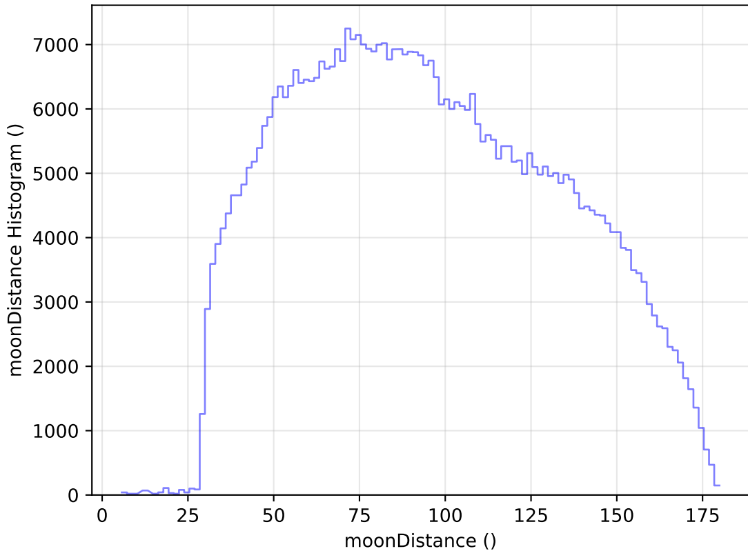
too_elab_r32_d3_gz_v3.4_10yrs All sky i band: moonDistance Histogram
