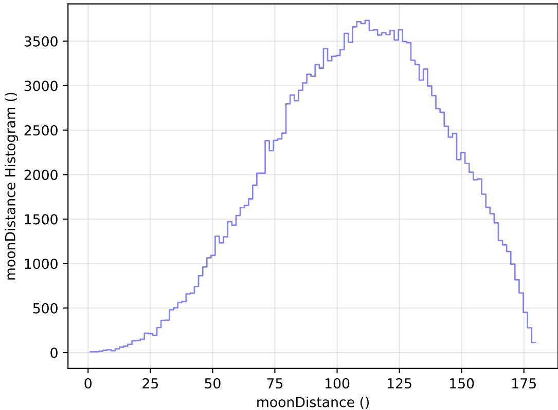
too_elab_r32_d3_gz_v3.4_10yrs All sky g band: moonDistance Histogram
