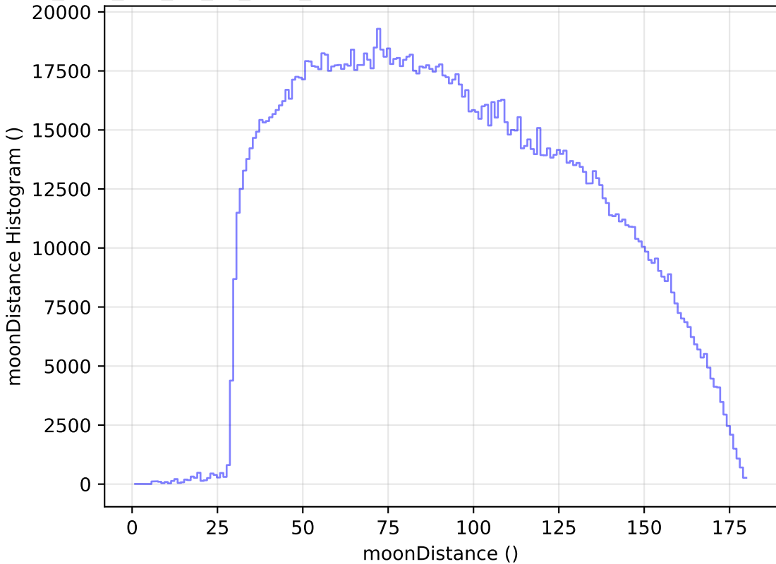
too_elab_r32_d3_gz_v3.4_10yrs All sky all bands: moonDistance Histogram
