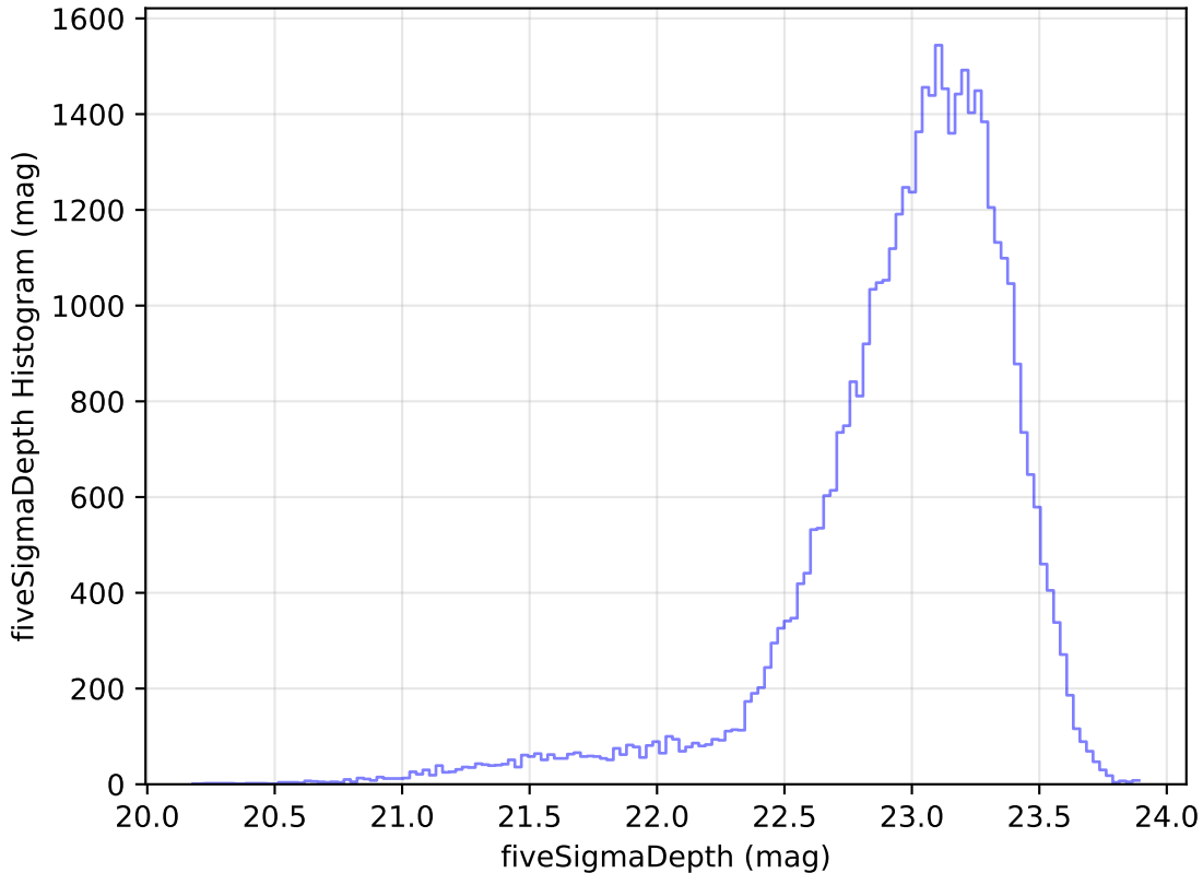
too_elab_r32_d3_gz_v3.4_10yrs Yr 1 z band: fiveSigmaDepth Histogram
