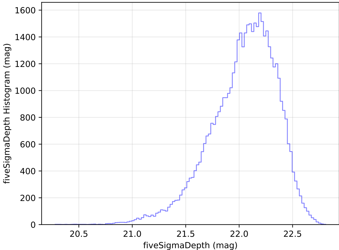
too_elab_r32_d3_gz_v3.4_10yrs Yr 1 y band: fiveSigmaDepth Histogram
