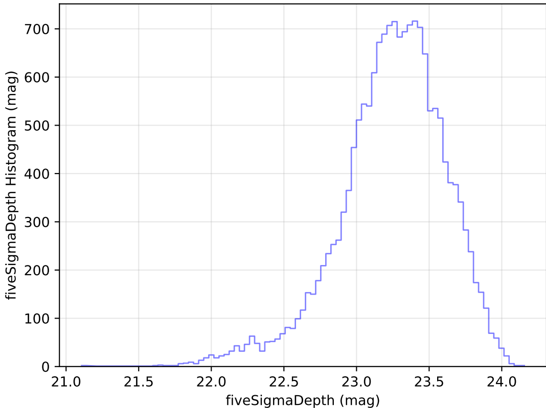
too_elab_r32_d3_gz_v3.4_10yrs Yr 1 u band: fiveSigmaDepth Histogram
