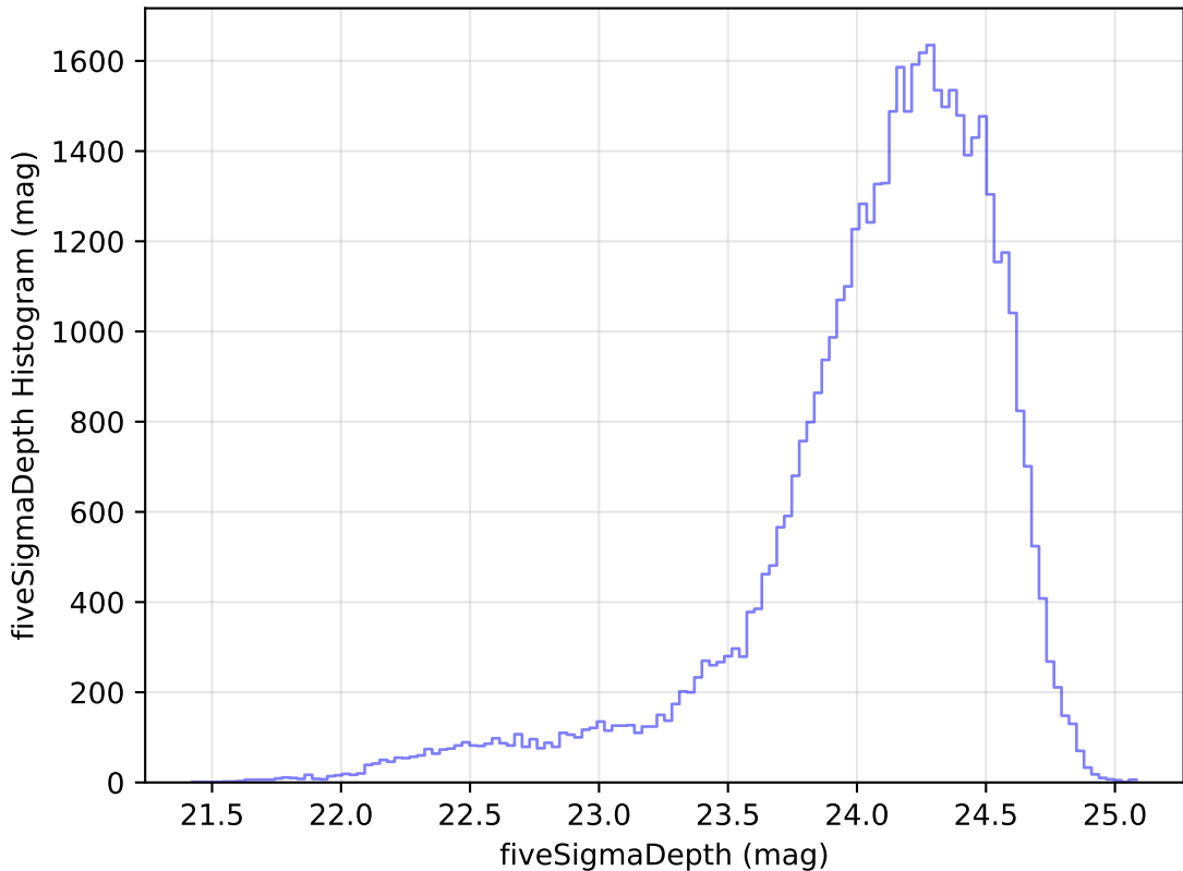
too_elab_r32_d3_gz_v3.4_10yrs Yr 1 r band: fiveSigmaDepth Histogram
