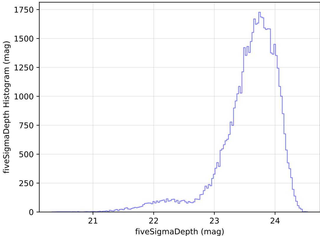
too_elab_r32_d3_gz_v3.4_10yrs Yr 1 i band: fiveSigmaDepth Histogram
