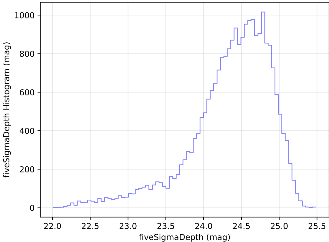
too_elab_r32_d3_gz_v3.4_10yrs Yr 1 g band: fiveSigmaDepth Histogram
