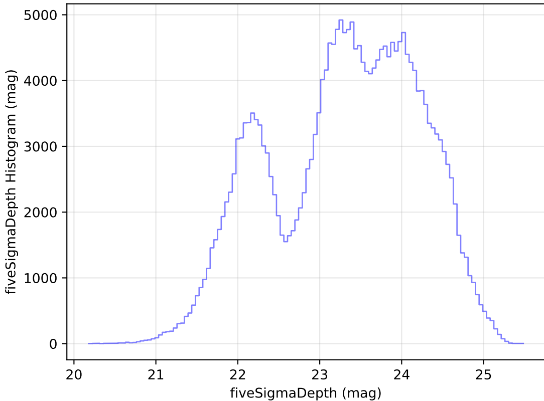
too_elab_r32_d3_gz_v3.4_10yrs Yr 1 all bands: fiveSigmaDepth Histogram
