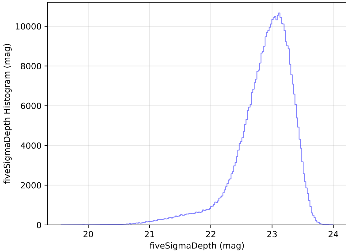
too_elab_r32_d3_gz_v3.4_10yrs WFD z band: fiveSigmaDepth Histogram
