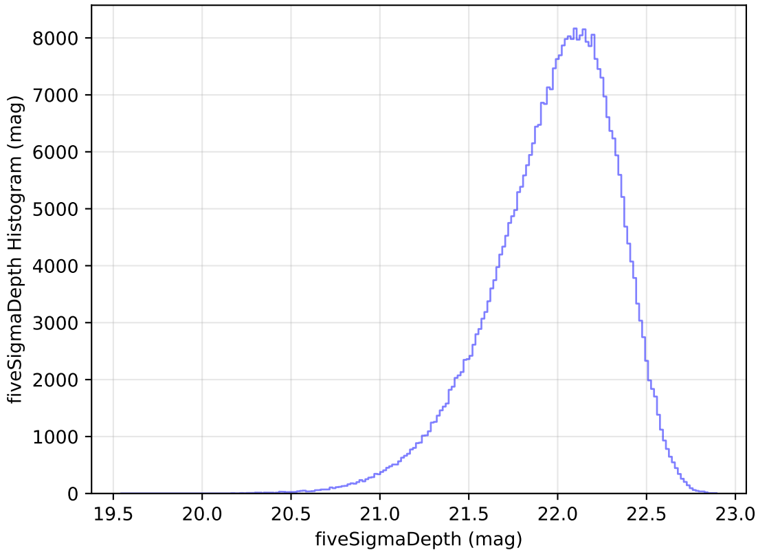
too_elab_r32_d3_gz_v3.4_10yrs WFD y band: fiveSigmaDepth Histogram
