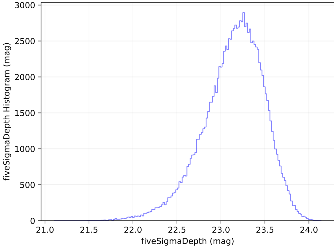
too_elab_r32_d3_gz_v3.4_10yrs WFD u band: fiveSigmaDepth Histogram
