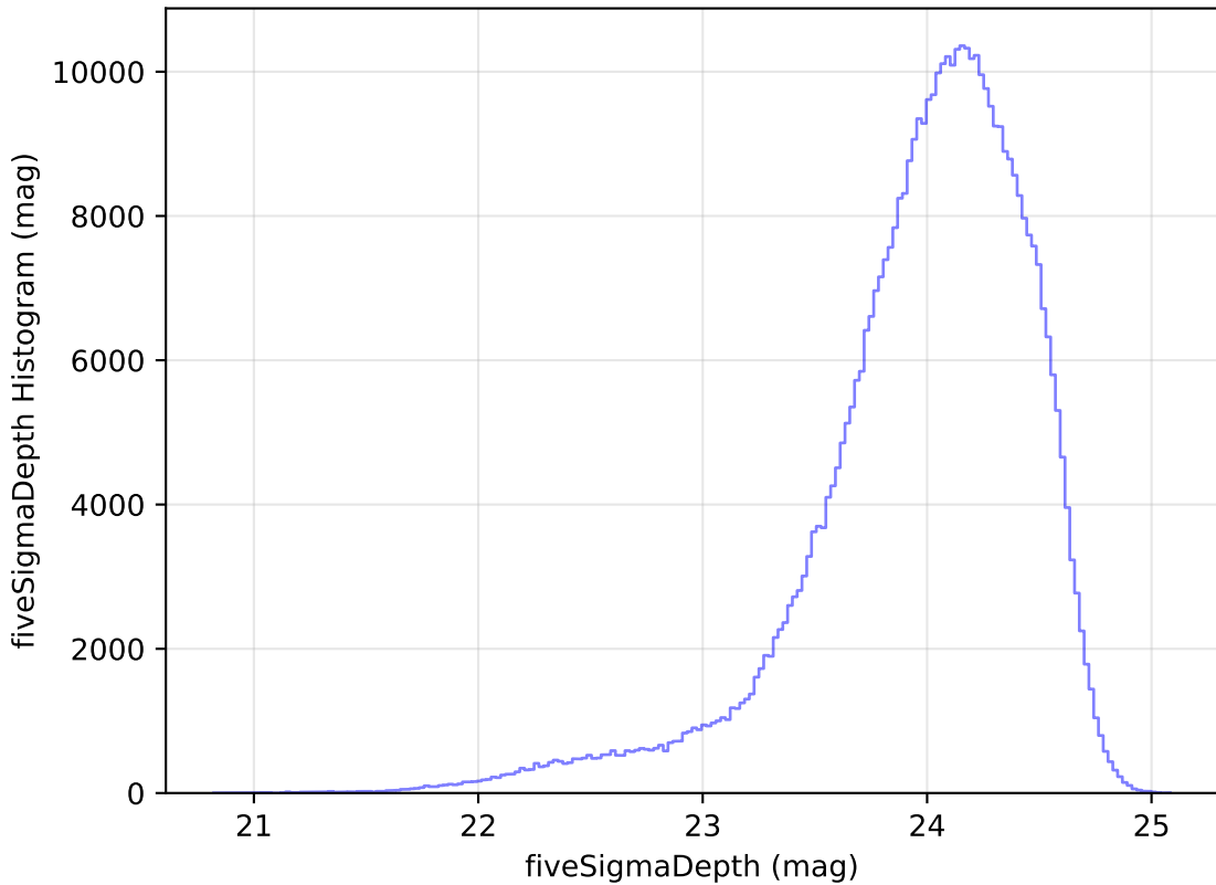
too_elab_r32_d3_gz_v3.4_10yrs WFD r band: fiveSigmaDepth Histogram
