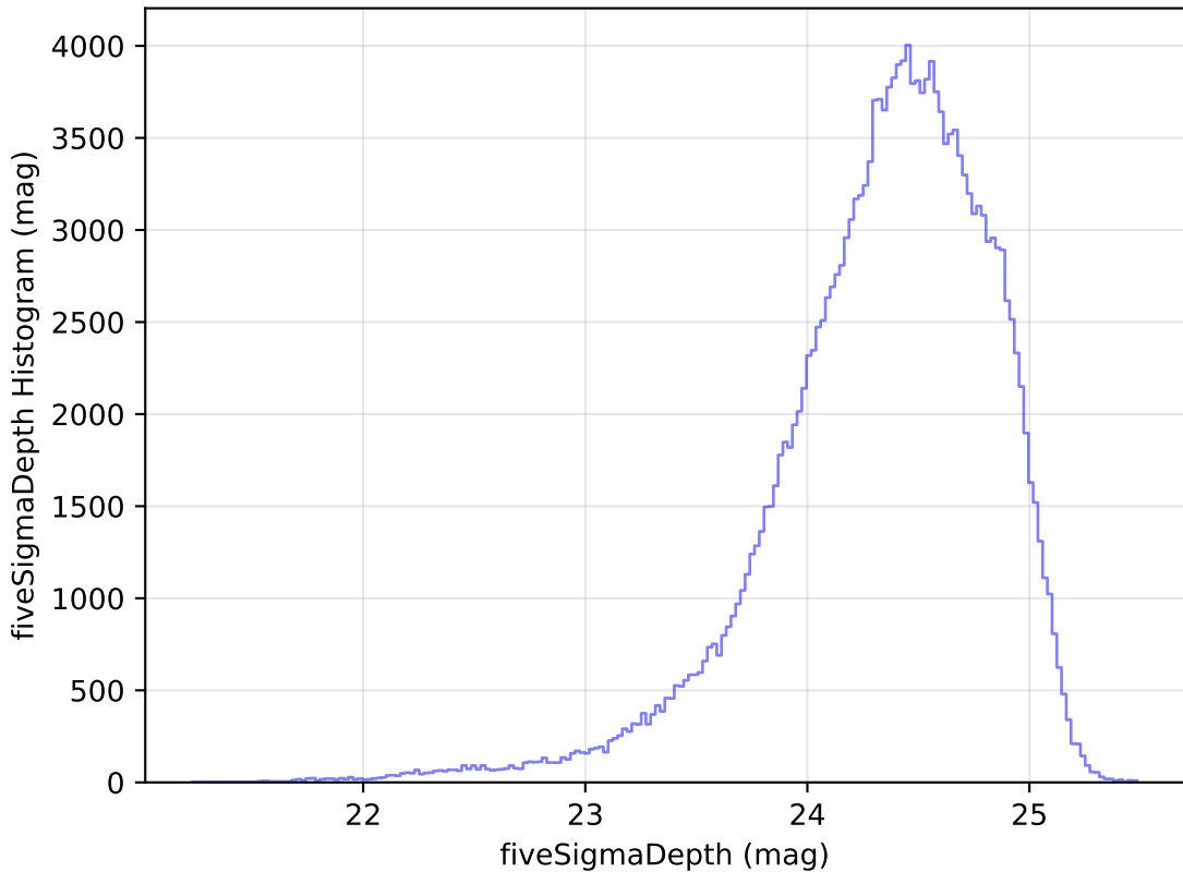
too_elab_r32_d3_gz_v3.4_10yrs WFD g band: fiveSigmaDepth Histogram
