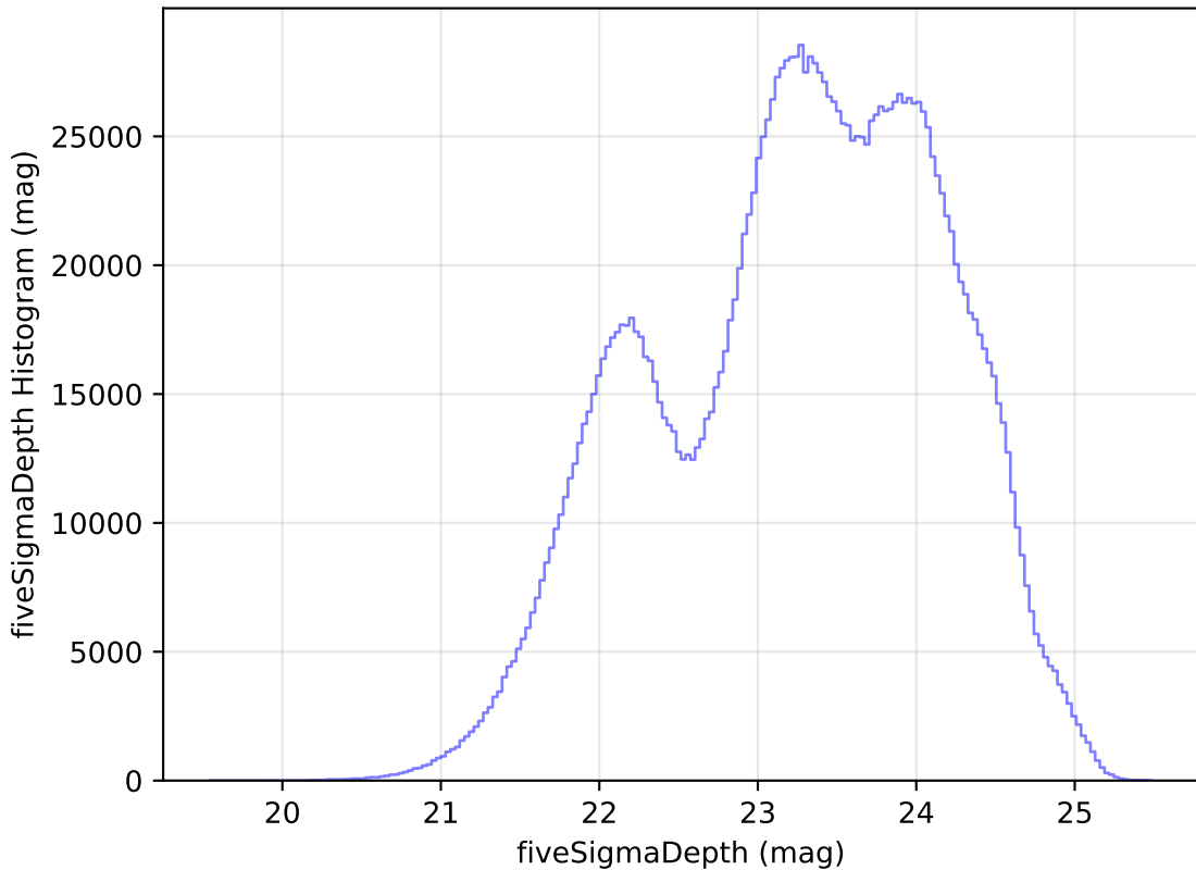
too_elab_r32_d3_gz_v3.4_10yrs WFD all bands: fiveSigmaDepth Histogram
