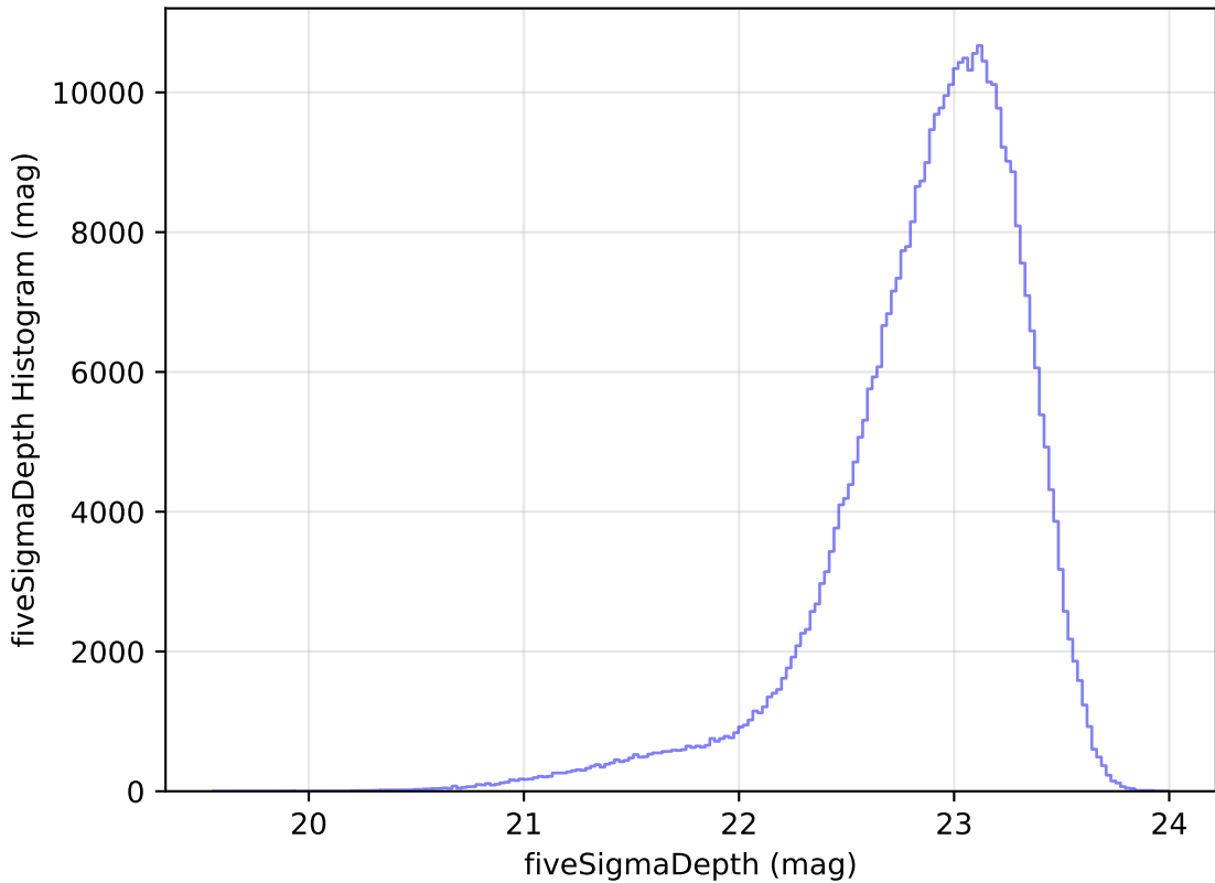
too_elab_r32_d3_gz_v3.4_10yrs All sky z band: fiveSigmaDepth Histogram
