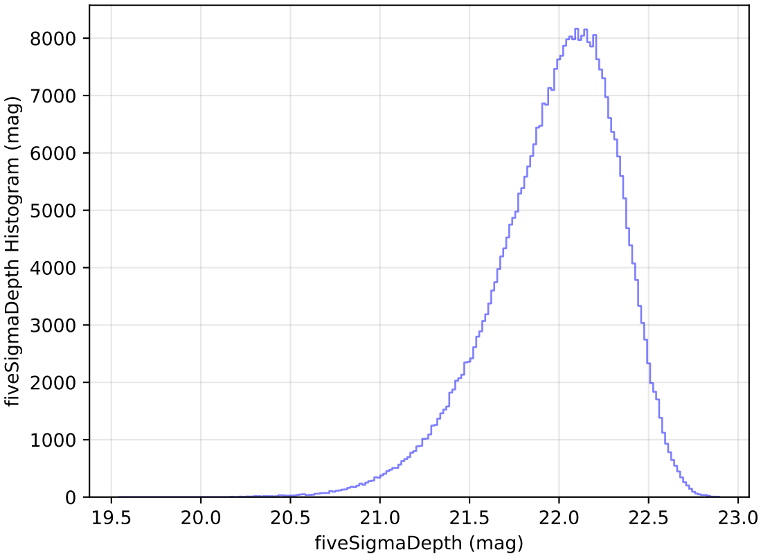
too_elab_r32_d3_gz_v3.4_10yrs All sky y band: fiveSigmaDepth Histogram
