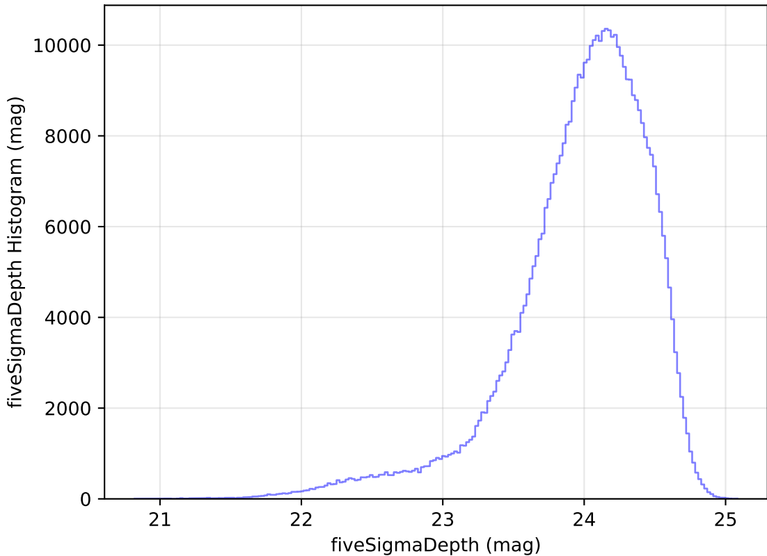
too_elab_r32_d3_gz_v3.4_10yrs All sky r band: fiveSigmaDepth Histogram
