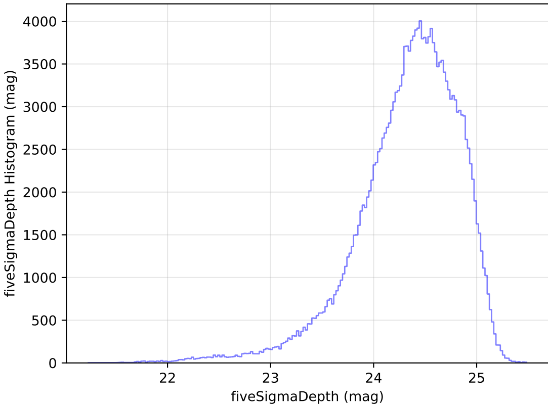
too_elab_r32_d3_gz_v3.4_10yrs All sky g band: fiveSigmaDepth Histogram
