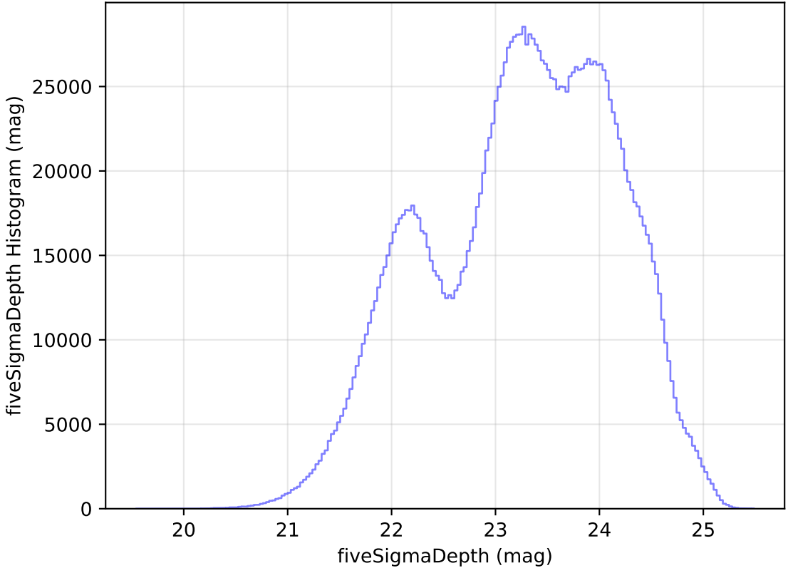
too_elab_r32_d3_gz_v3.4_10yrs All sky all bands: fiveSigmaDepth Histogram
