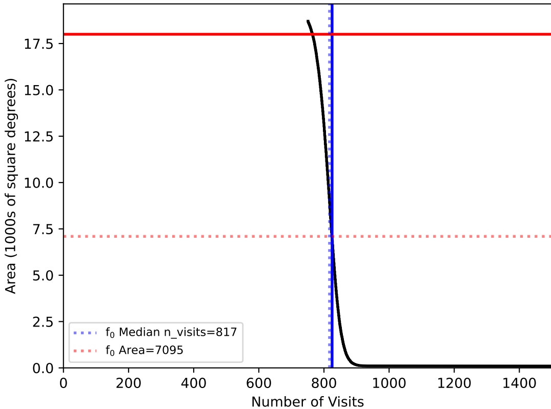
too_elab_r32_d3_gz_v3.4_10yrs WFD: fO
