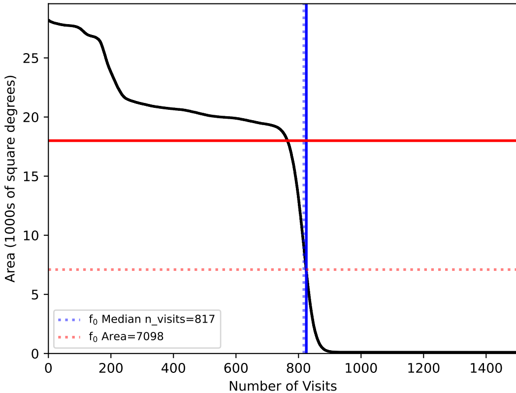
too_elab_r32_d3_gz_v3.4_10yrs All sky: f0
