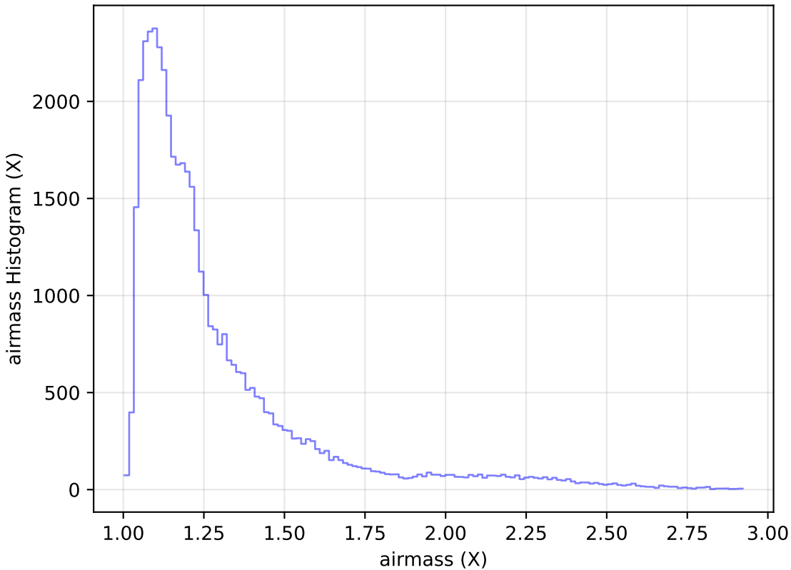
too_elab_r32_d3_gz_v3.4_10yrs Yr 1 z band: airmass Histogram
