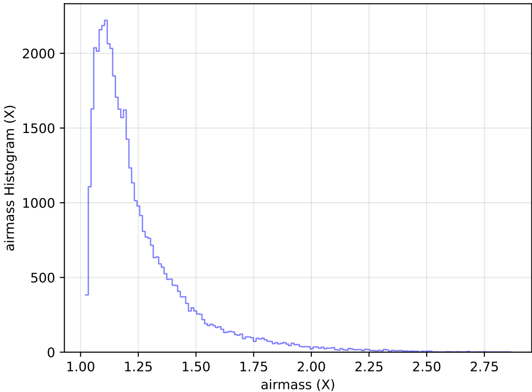
too_elab_r32_d3_gz_v3.4_10yrs Yr 1 y band: airmass Histogram
