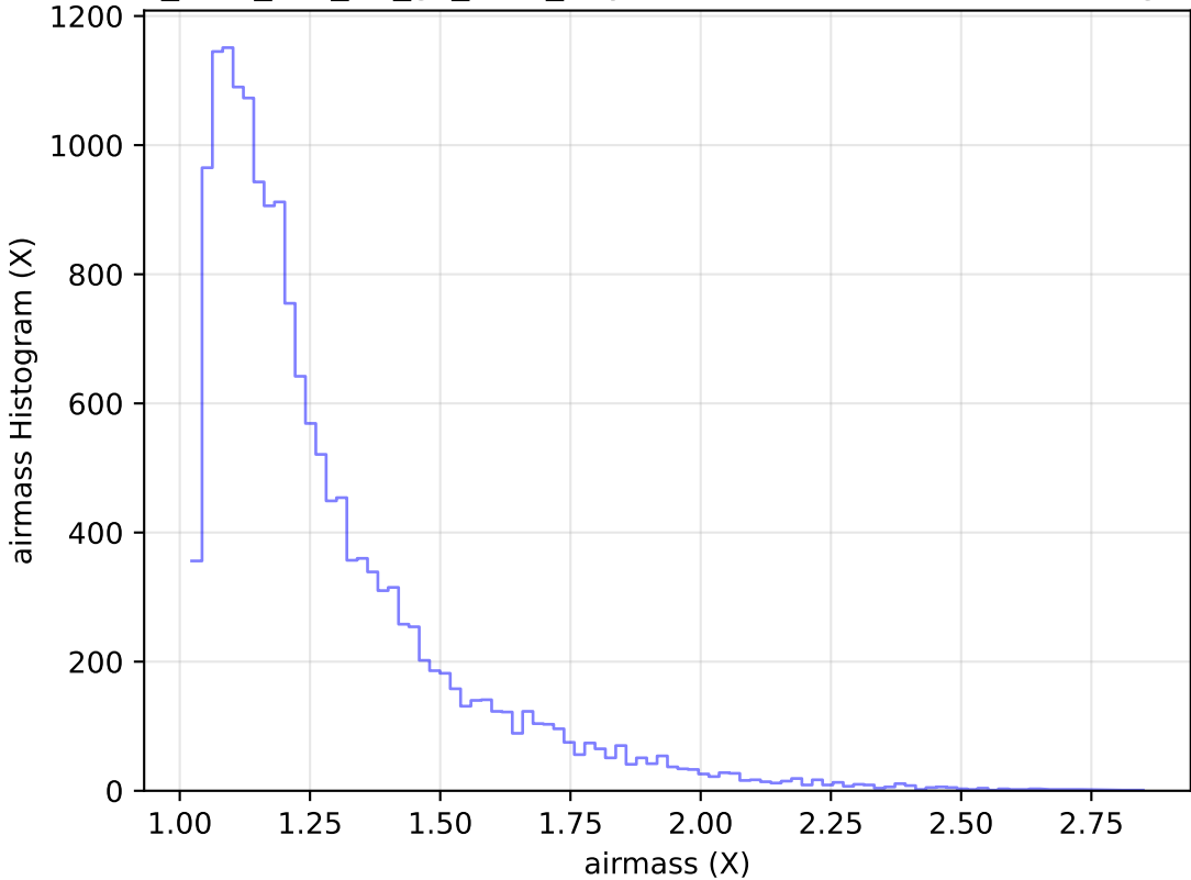
too_elab_r32_d3_gz_v3.4_10yrs Yr 1 u band: airmass Histogram
